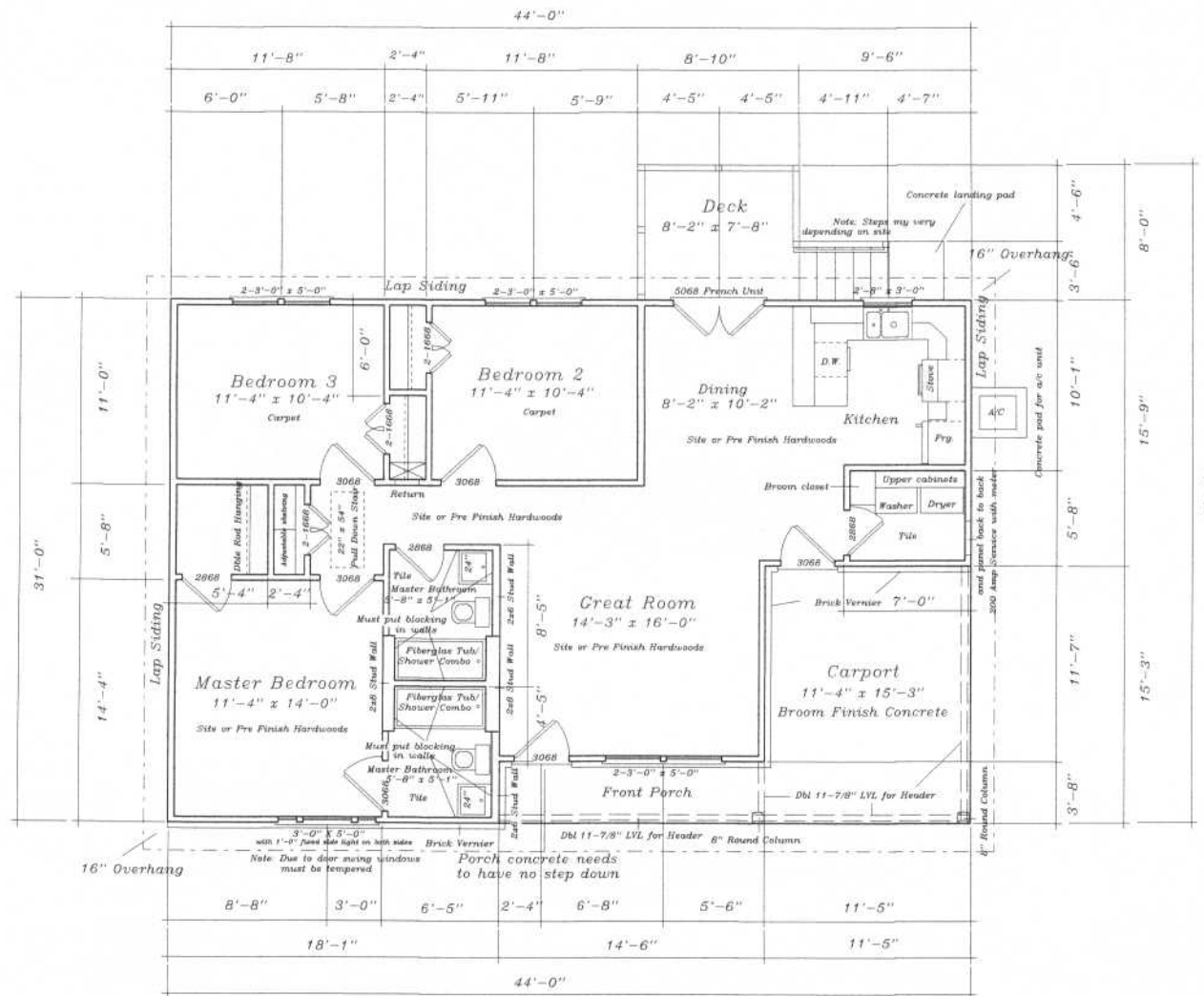
Dimension Plan
