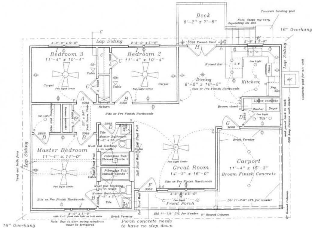
Floor Plan 1,138 sqft. Heated Space
