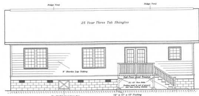
Rear Elevation
