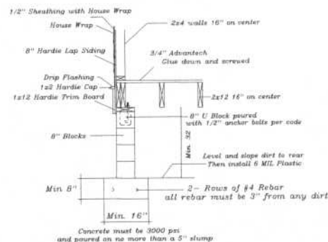
Section B
