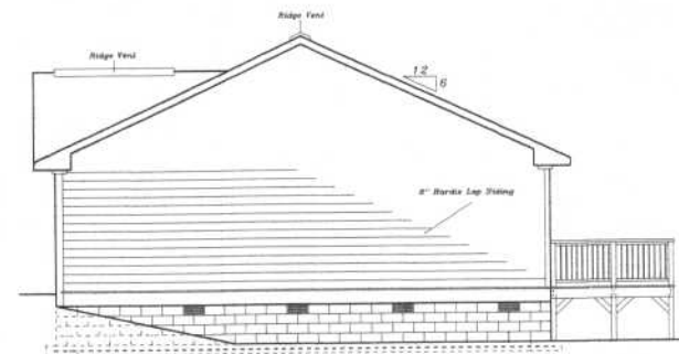
Right Side Elevations
