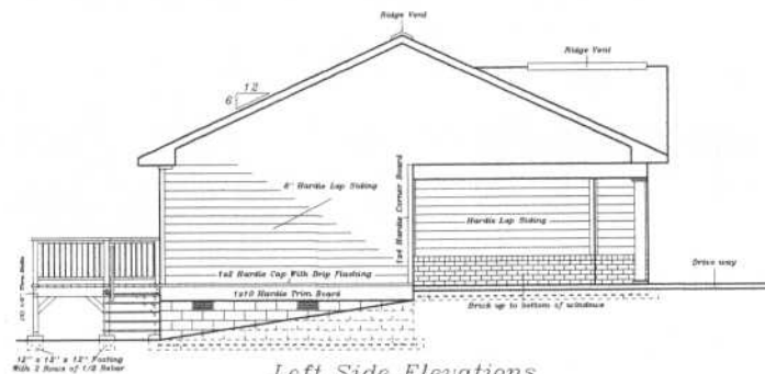
Left Side Elevations
