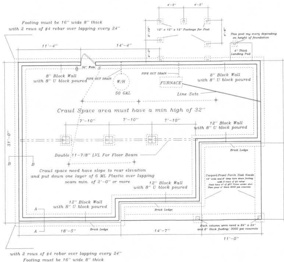
Foundation Plan
