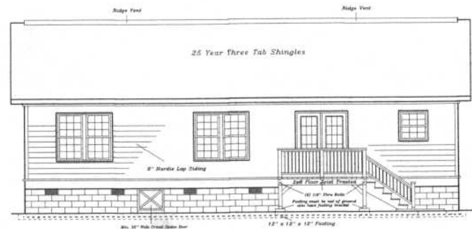
Rear Elevation
