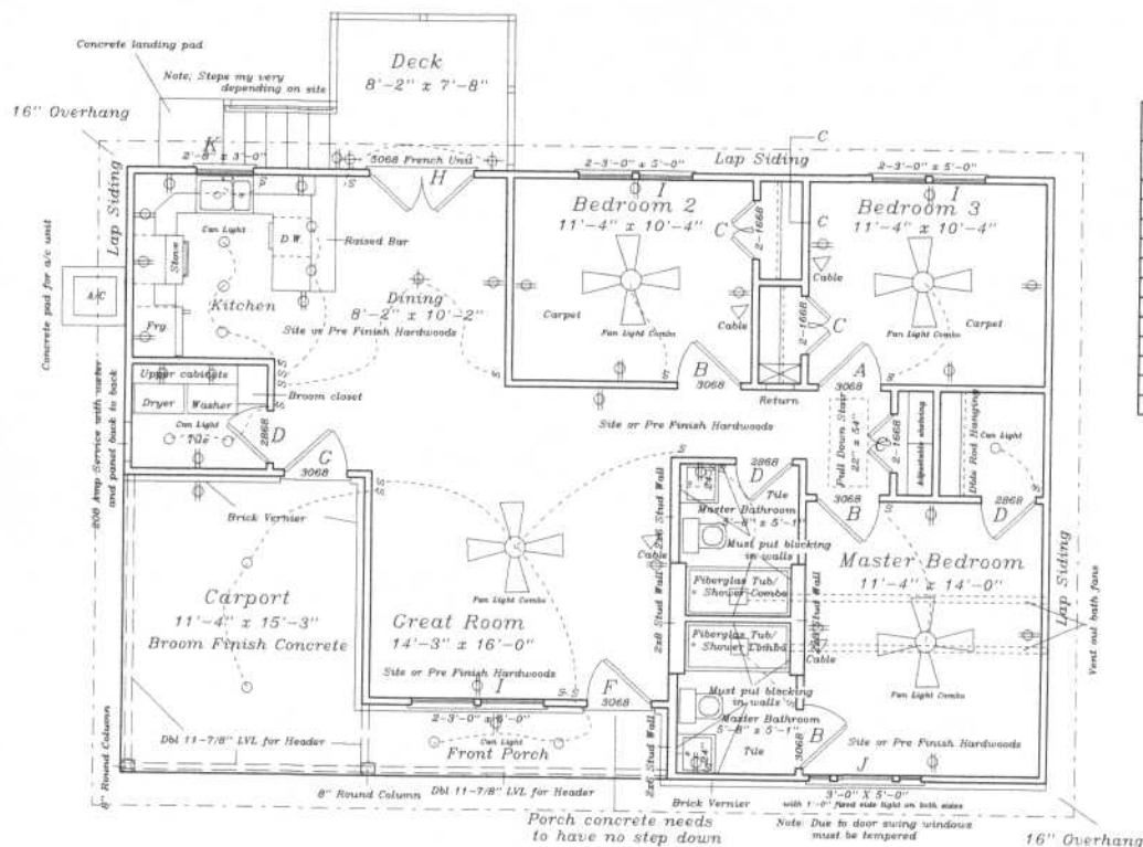
Floor Plan 1,138 sqft. Heated Space
