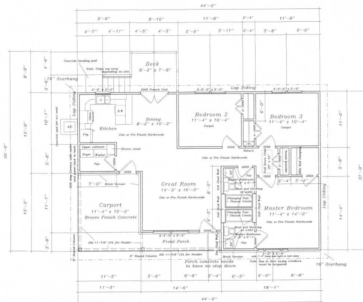
Dimension Plan 1,138 sqft. Heated Space
