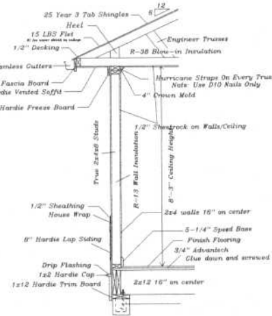
Section C Scale N/A
