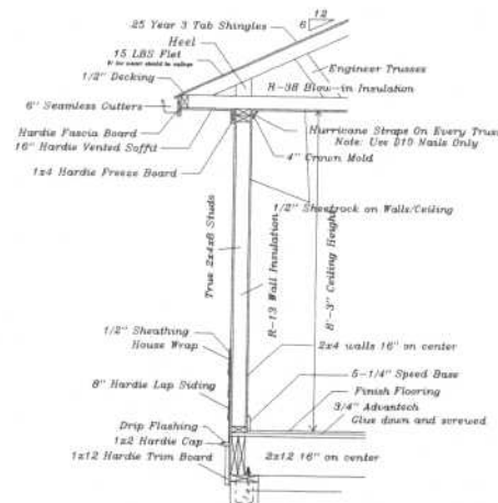
Section C Scale N/A
